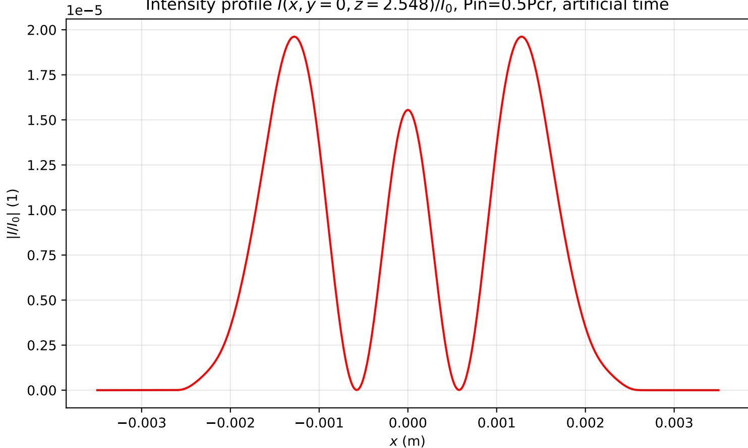
Intensity profile I(x, y = 0, z = 2.548)/I_0 , P_{in}=0.5P_{cr} , artificial time
